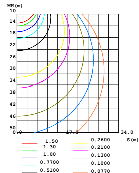
CO PLANE ISOLUX DIAGRAM (UNIT: lx)
